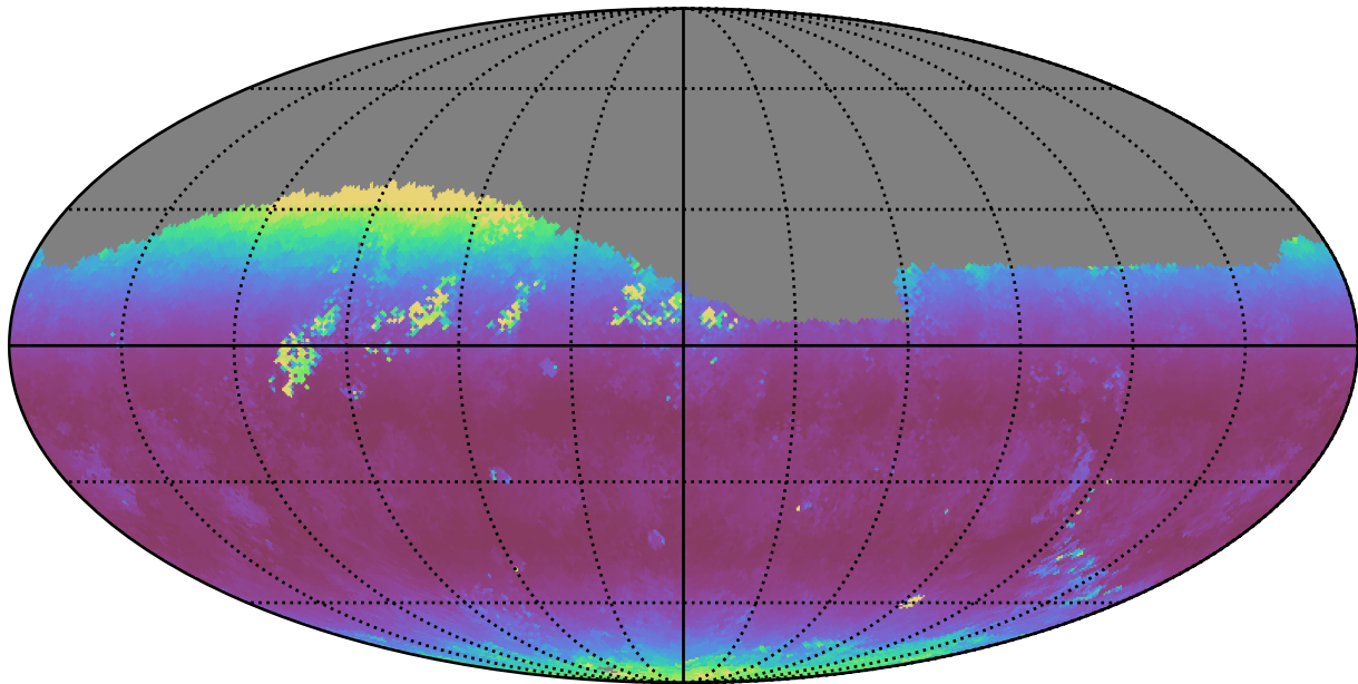
baseline_v3.3_10yrs Yr 1 r band: Median airmass
