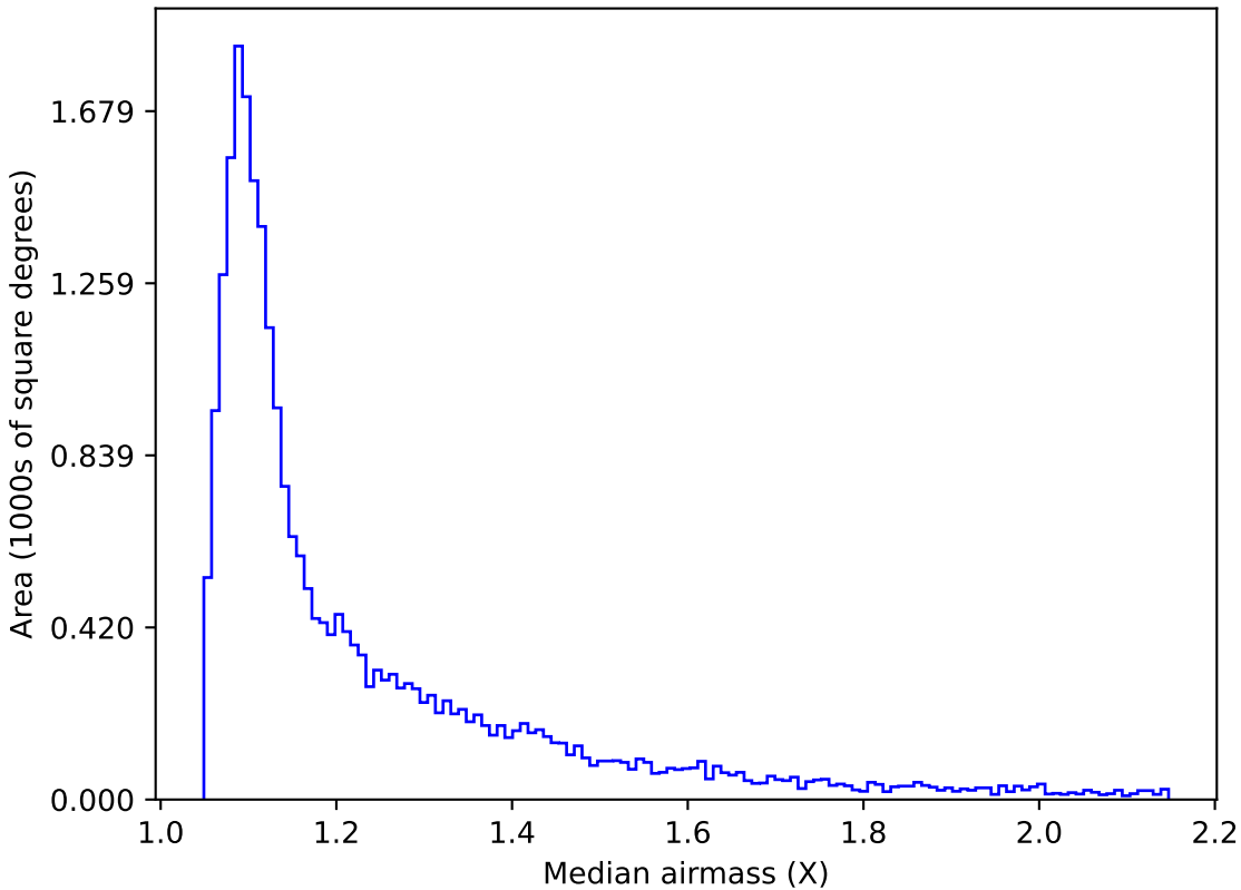
baseline_v3.3_10yrs Yr 1 r band: Median airmass
