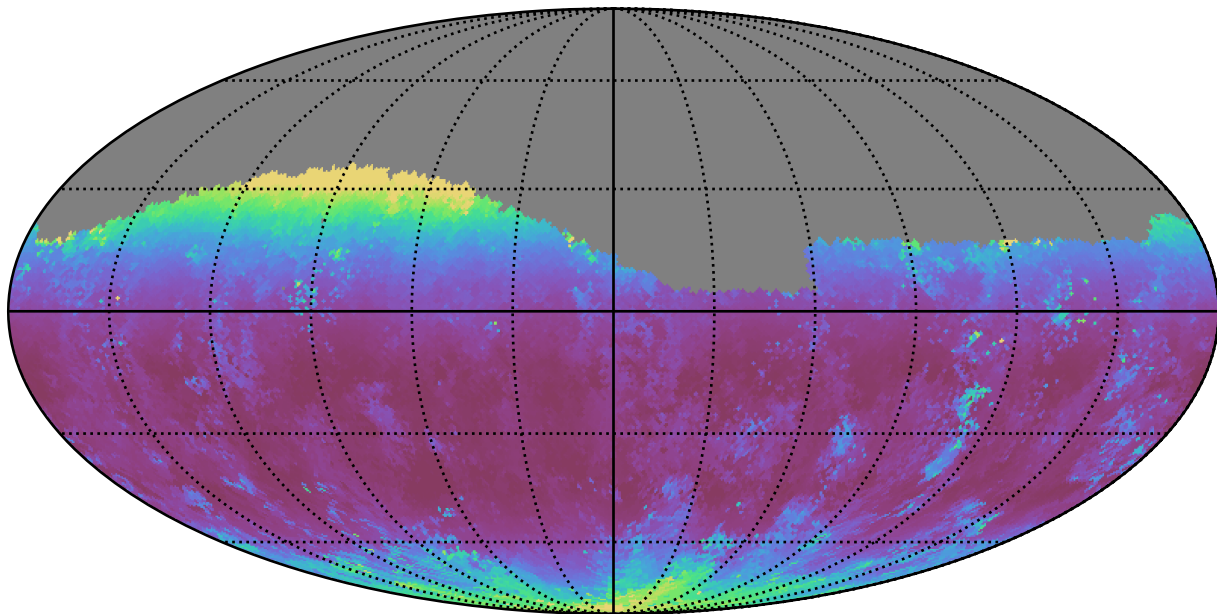
baseline_v3.3_10yrs Yr 1 g band: Median airmass
