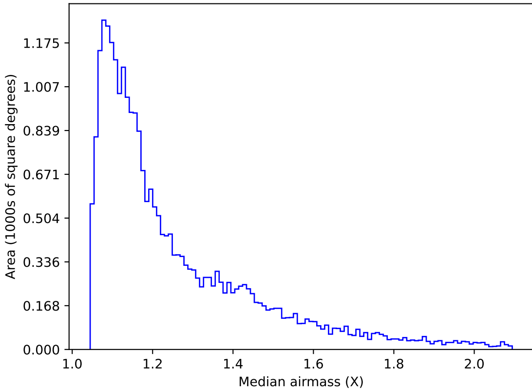
baseline_v3.3_10yrs Yr 1 g band: Median airmass
