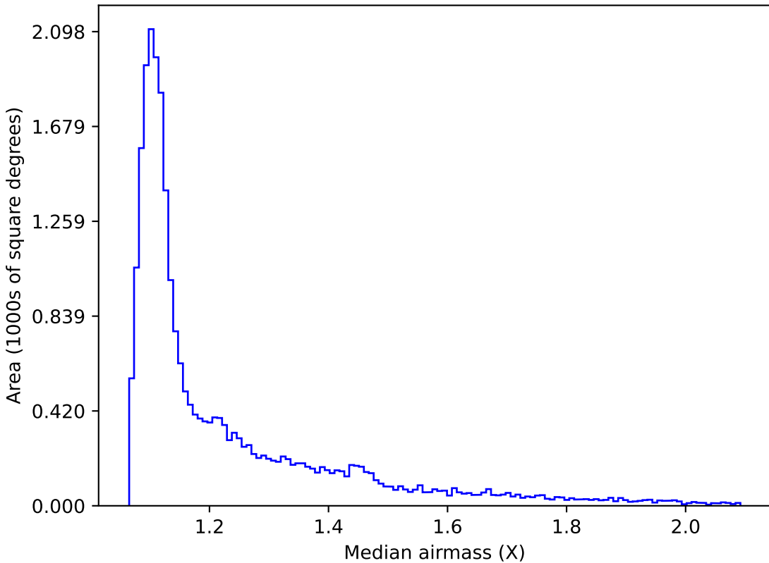
baseline_v3.3_10yrs Yr 1 all bands: Median airmass
