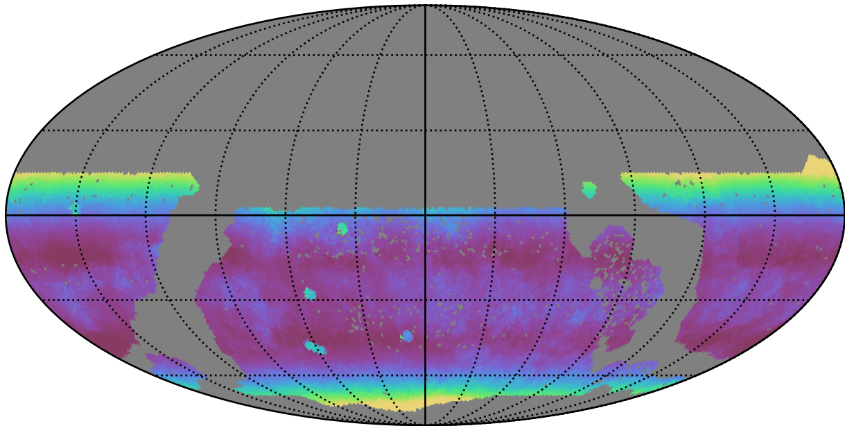
baseline_v3.3_10yrs WFD z band: Median airmass
