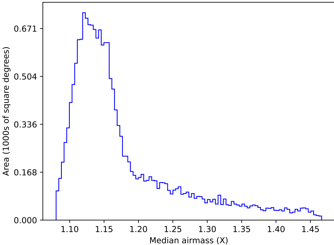
baseline_v3.3_10yrs WFD z band: Median airmass
