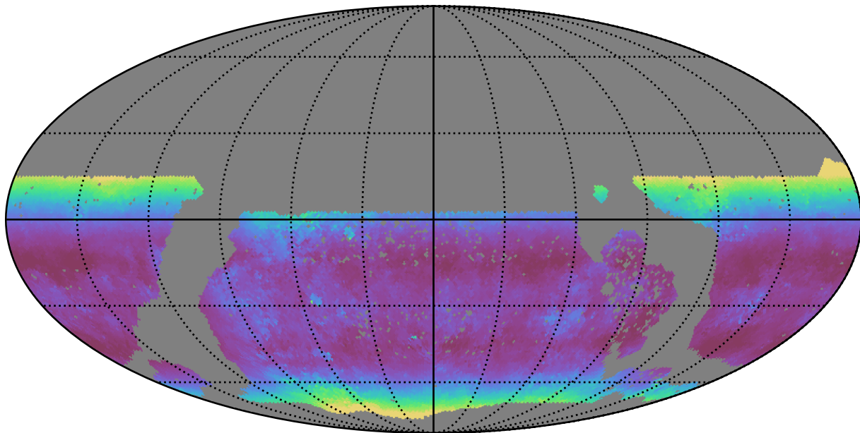
baseline_v3.3_10yrs WFD u band: Median airmass
