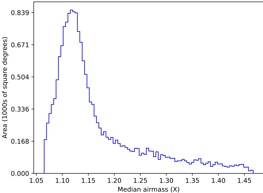
baseline_v3.3_10yrs WFD u band: Median airmass
