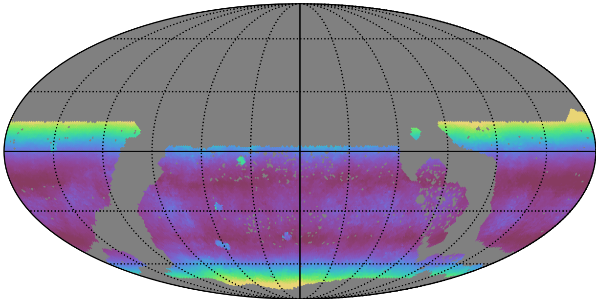
baseline_v3.3_10yrs WFD r band: Median airmass
