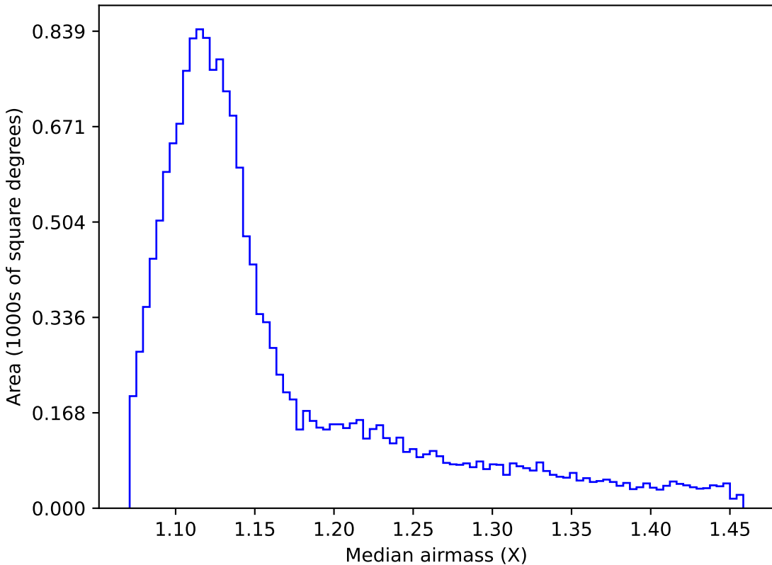
baseline_v3.3_10yrs WFD r band: Median airmass
