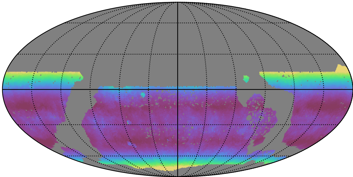
baseline_v3.3_10yrs WFD i band: Median airmass
