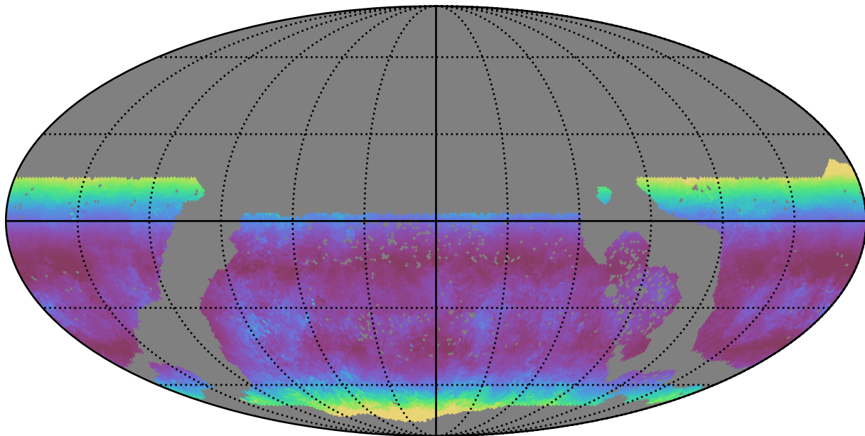
baseline_v3.3_10yrs WFD g band: Median airmass
