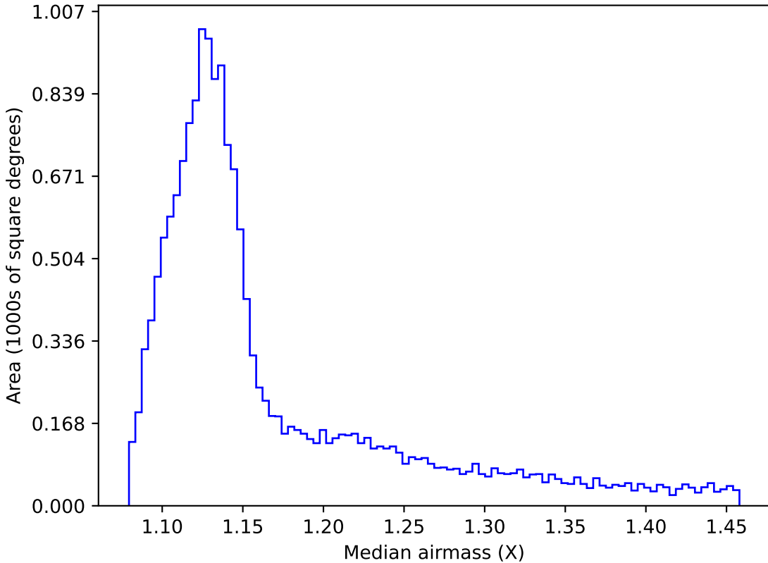
baseline_v3.3_10yrs WFD all bands: Median airmass
