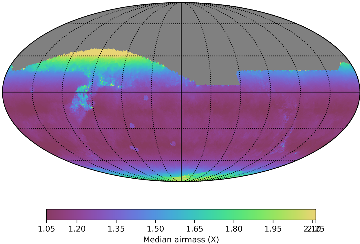
baseline_v3.3_10yrs All sky z band: Median airmass
