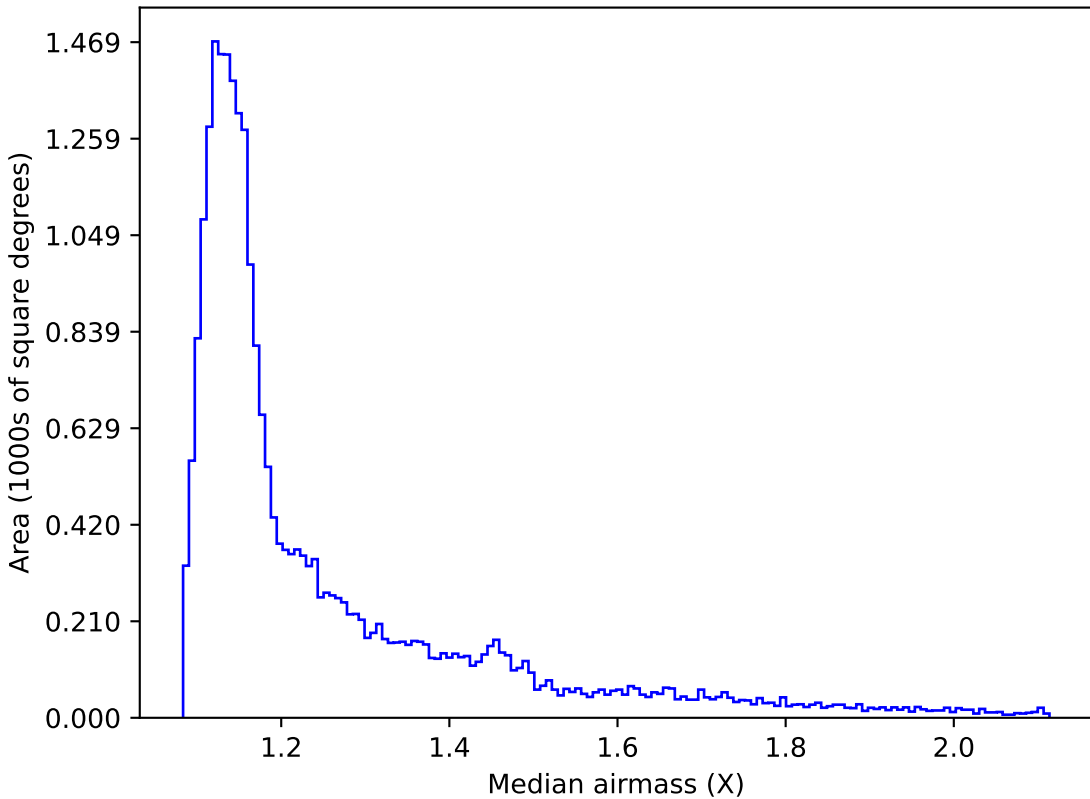
baseline_v3.3_10yrs All sky z band: Median airmass
