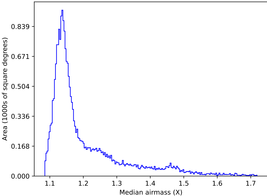
baseline_v3.3_10yrs All sky y band: Median airmass
