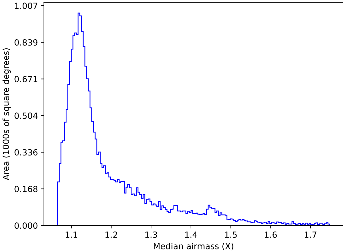
baseline_v3.3_10yrs All sky u band: Median airmass
