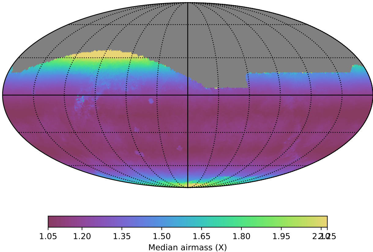
baseline_v3.3_10yrs All sky r band: Median airmass
