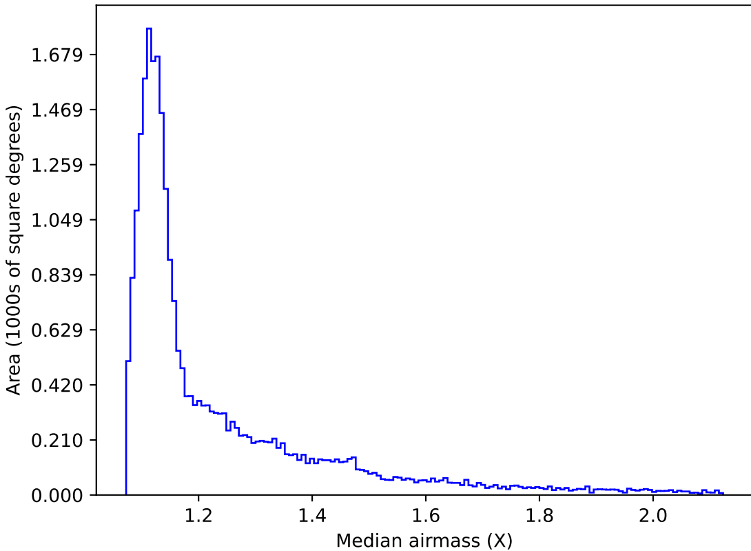
baseline_v3.3_10yrs All sky r band: Median airmass
