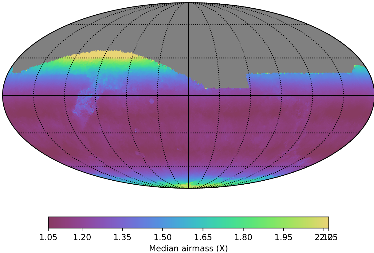
baseline_v3.3_10yrs All sky i band: Median airmass
