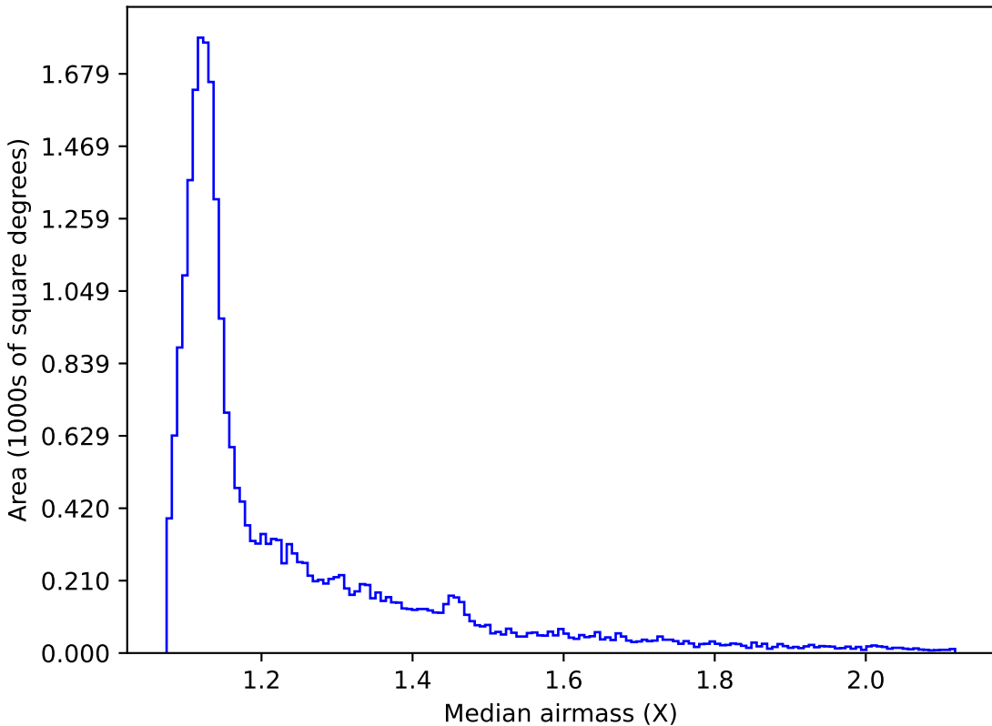
baseline_v3.3_10yrs All sky i band: Median airmass
