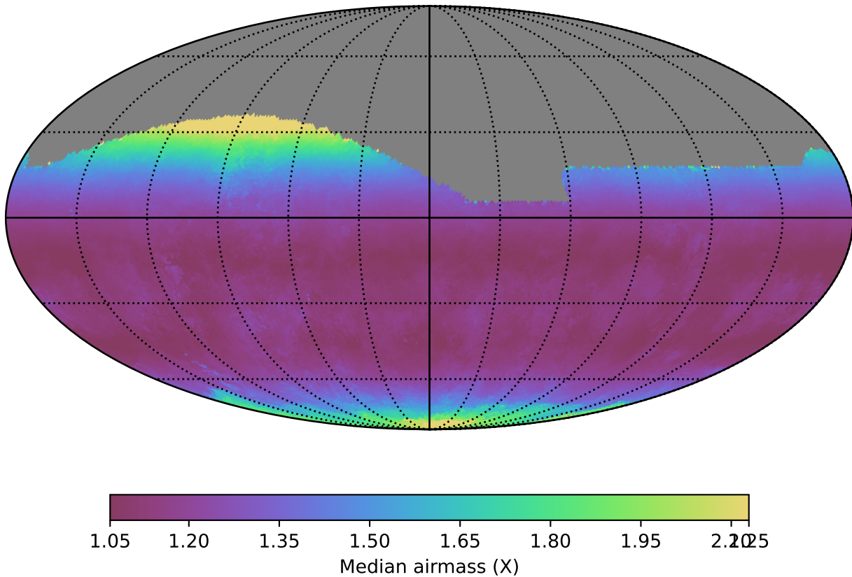
baseline_v3.3_10yrs All sky g band: Median airmass
