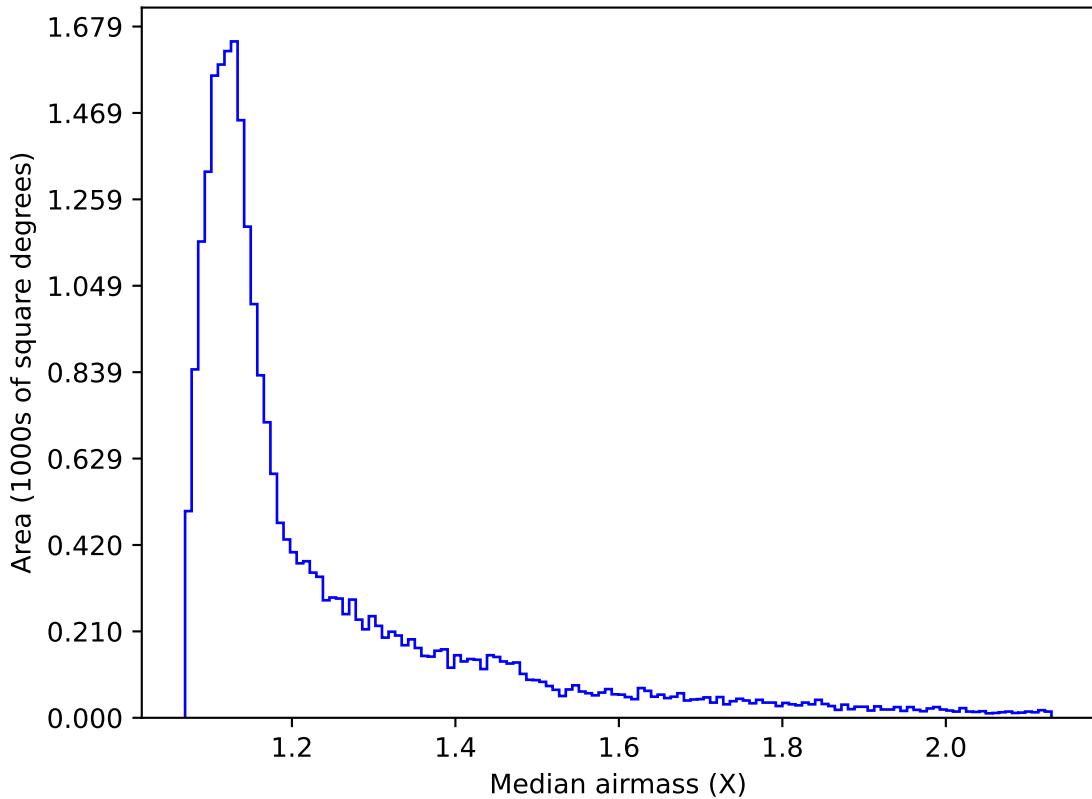
baseline_v3.3_10yrs All sky g band: Median airmass
