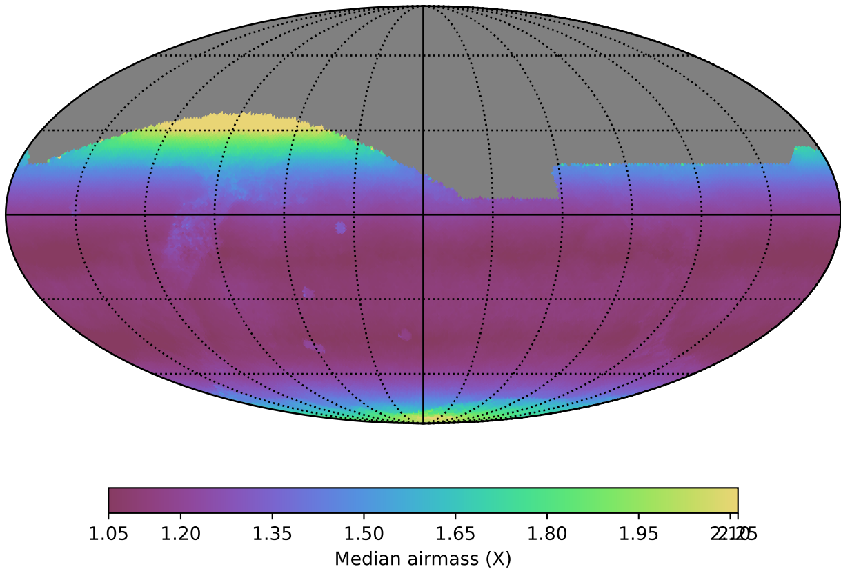
baseline_v3.3_10yrs All sky all bands: Median airmass
