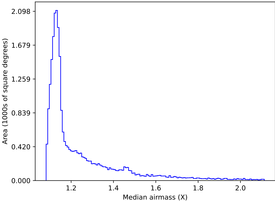
baseline_v3.3_10yrs All sky all bands: Median airmass
