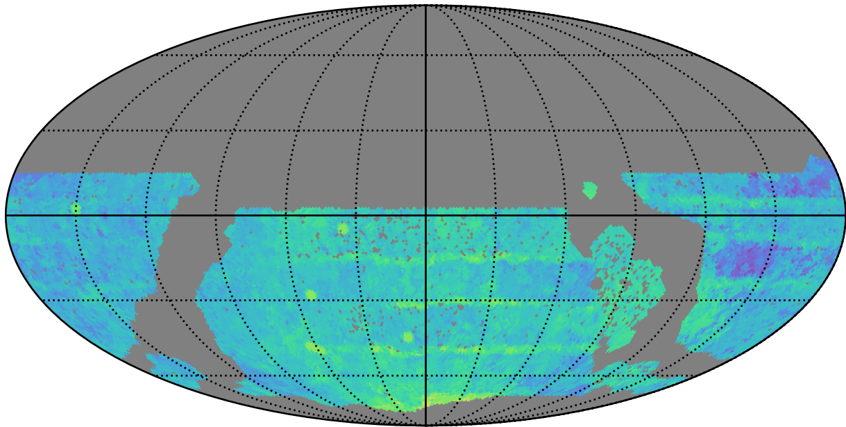
baseline_v3.3_10yrs WFD z band: Median Season Length
