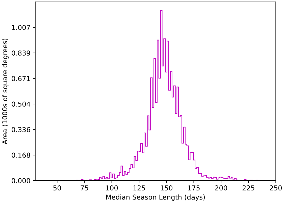
baseline_v3.3_10yrs WFD z band: Median Season Length
