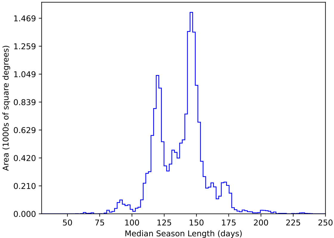
baseline_v3.3_10yrs WFD y band: Median Season Length
