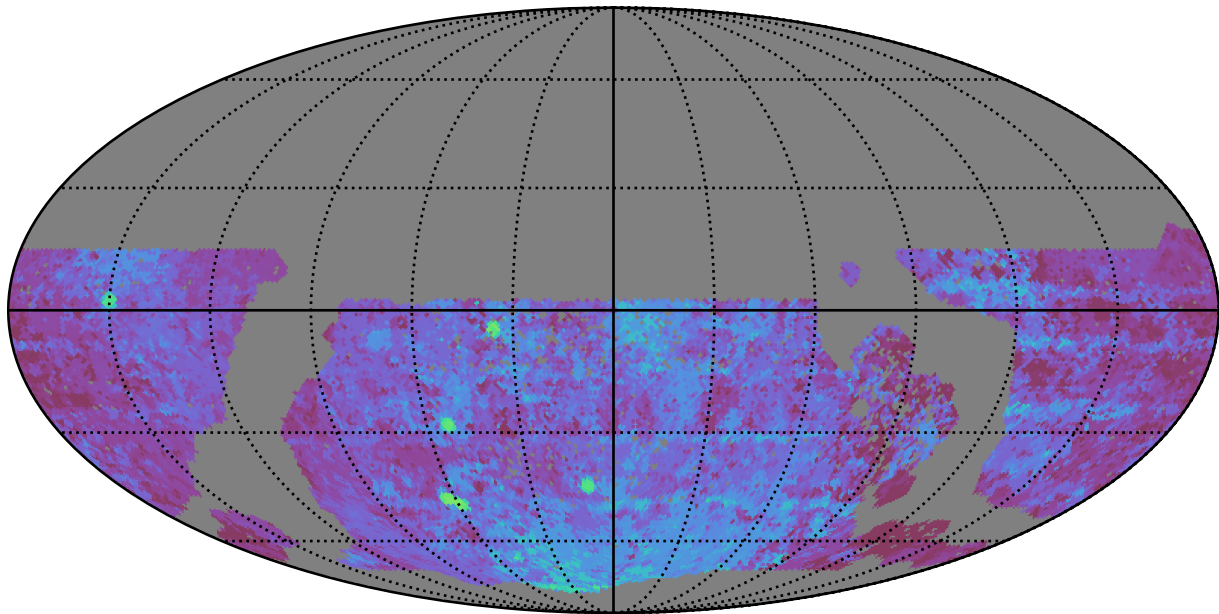
baseline_v3.3_10yrs WFD u band: Median Season Length
