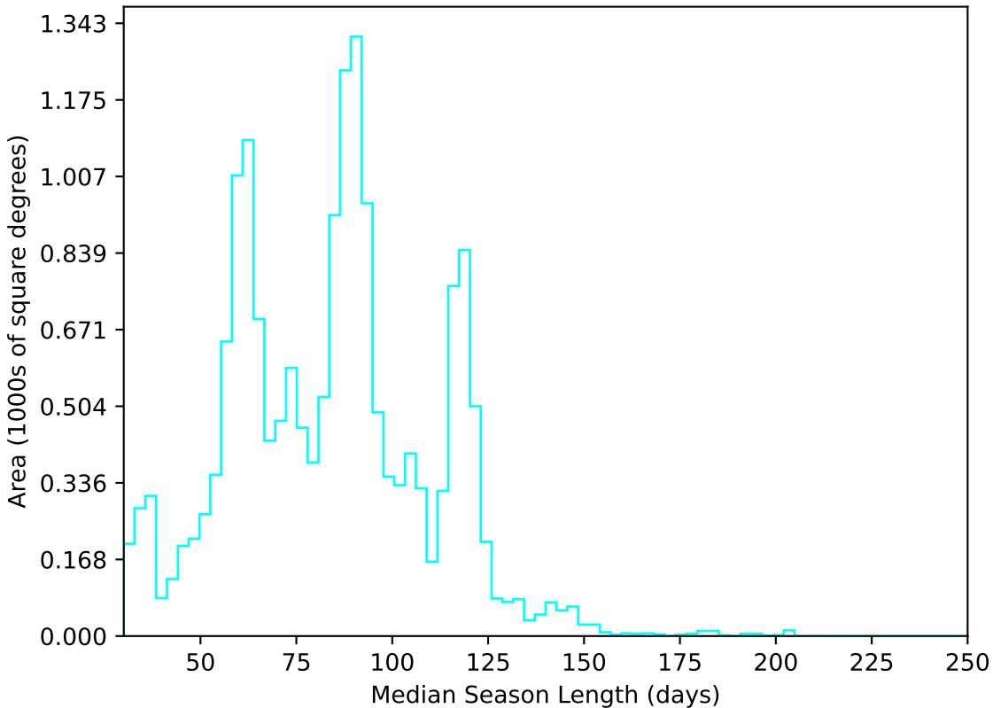
baseline_v3.3_10yrs WFD u band: Median Season Length
