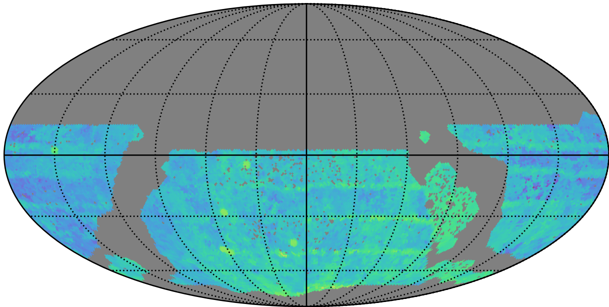
baseline_v3.3_10yrs WFD r band: Median Season Length
