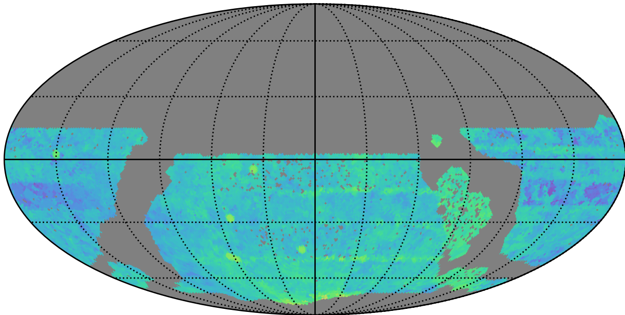
baseline_v3.3_10yrs WFD i band: Median Season Length
