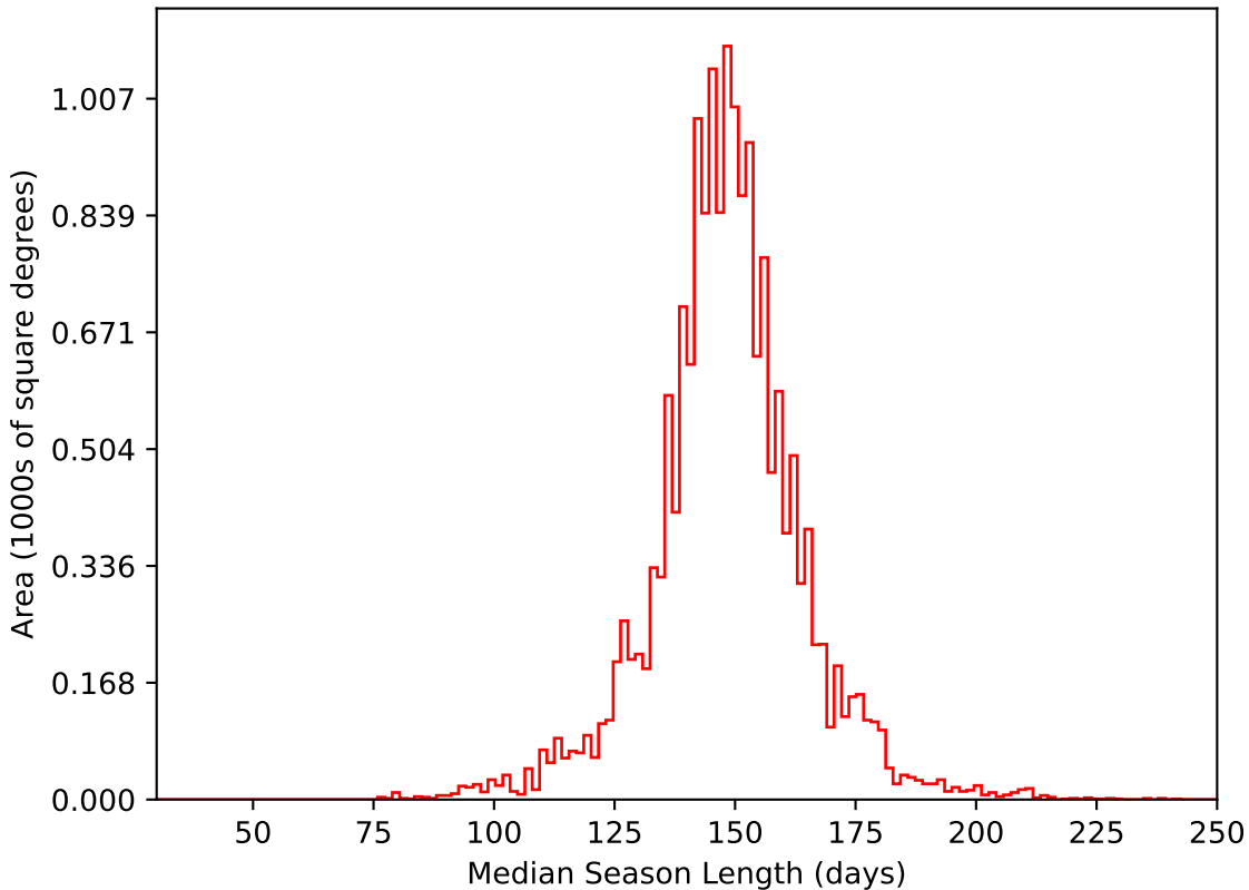
baseline_v3.3_10yrs WFD i band: Median Season Length
