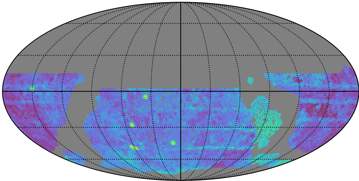
baseline_v3.3_10yrs WFD g band: Median Season Length
