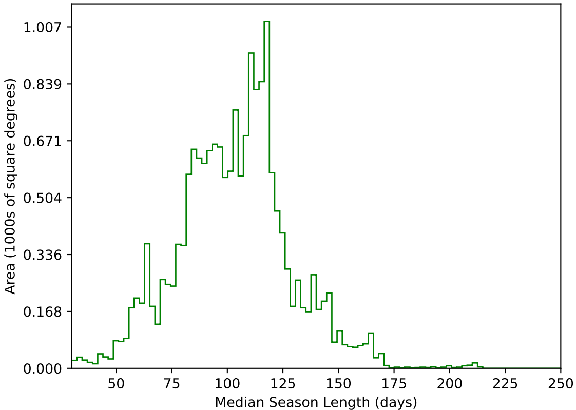
baseline_v3.3_10yrs WFD g band: Median Season Length
