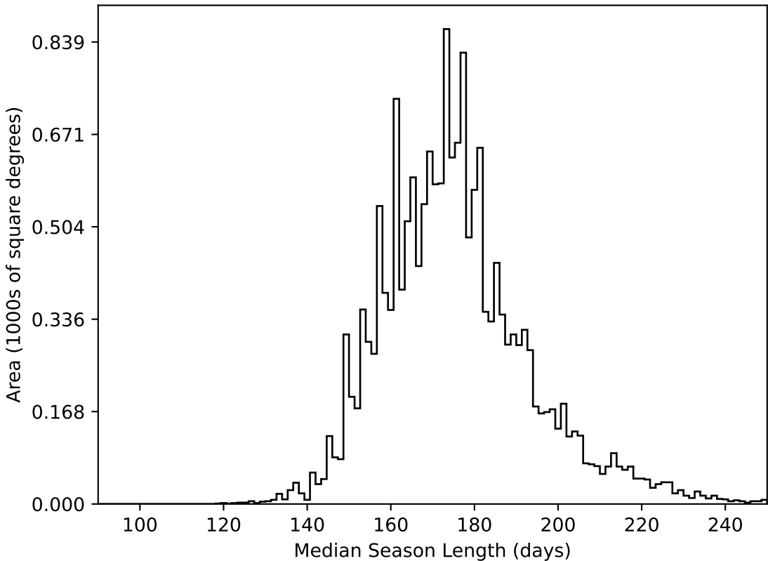
baseline_v3.3_10yrs WFD all bands: Median Season Length
