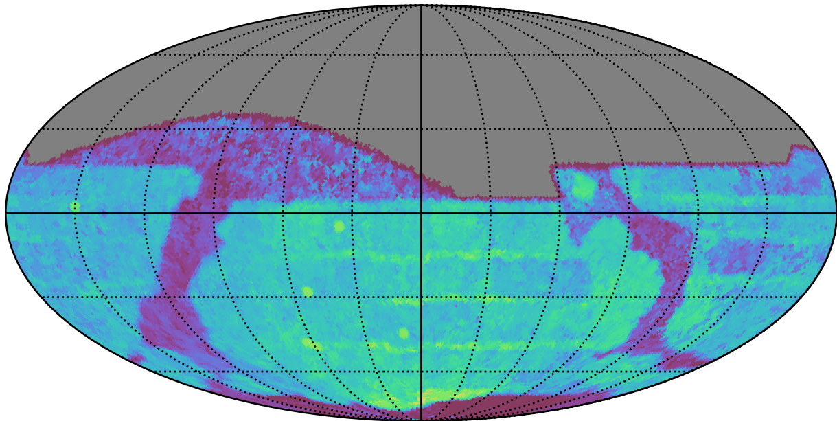
baseline_v3.3_10yrs All sky z band: Median Season Length
