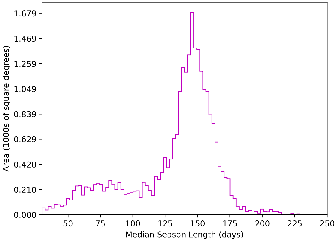
baseline_v3.3_10yrs All sky z band: Median Season Length
