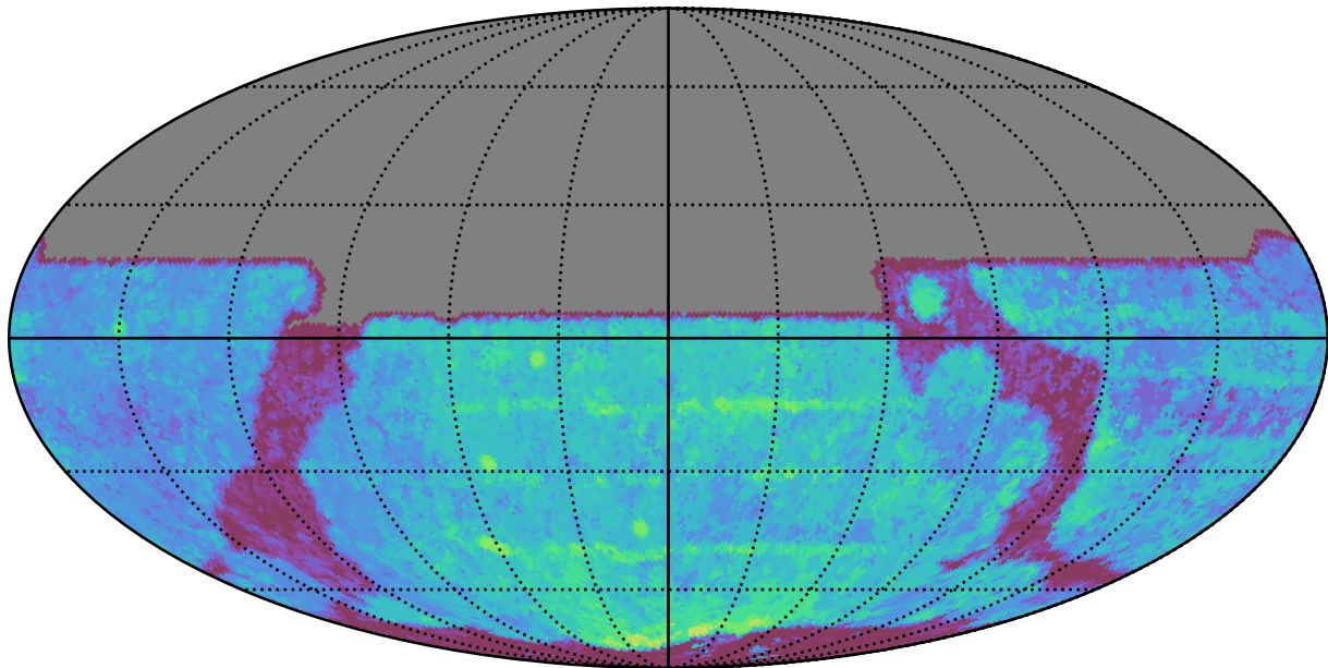
baseline_v3.3_10yrs All sky y band: Median Season Length
