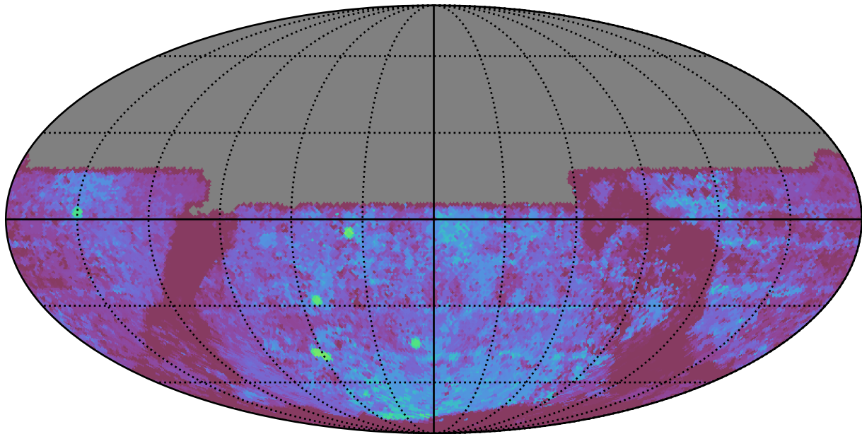
baseline_v3.3_10yrs All sky u band: Median Season Length
