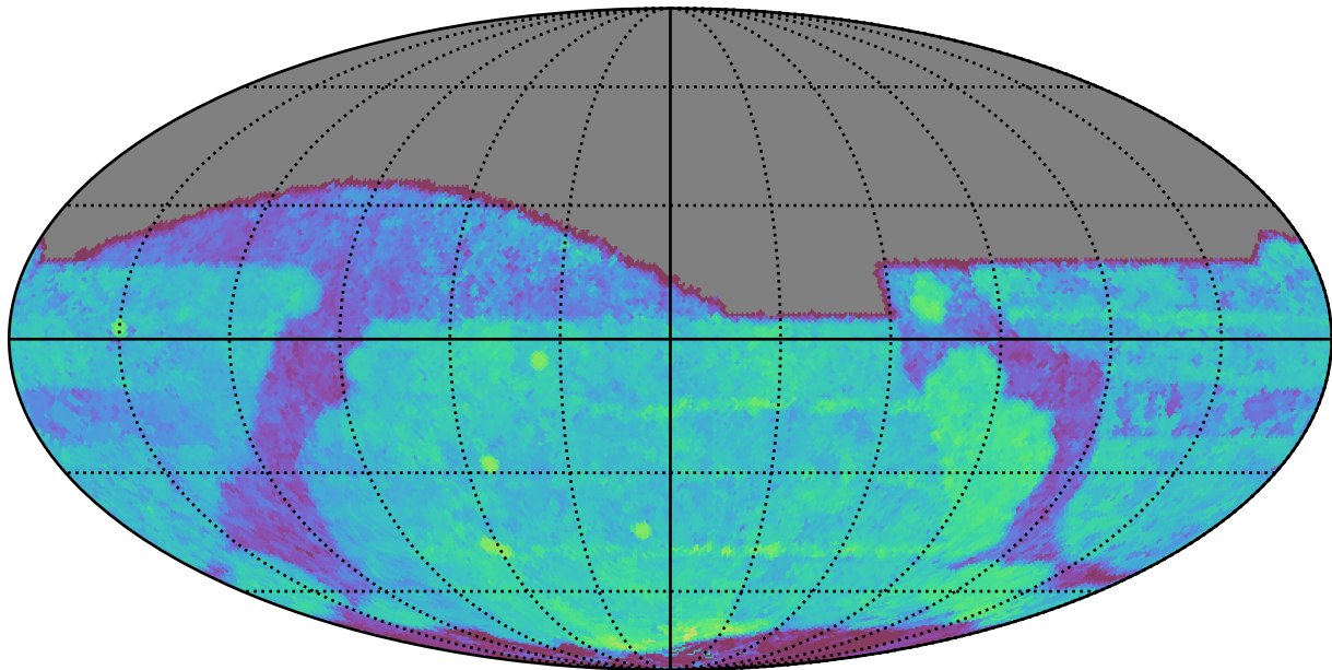
baseline_v3.3_10yrs All sky i band: Median Season Length
