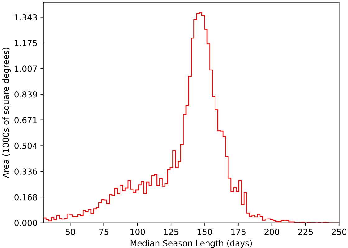
baseline_v3.3_10yrs All sky i band: Median Season Length
