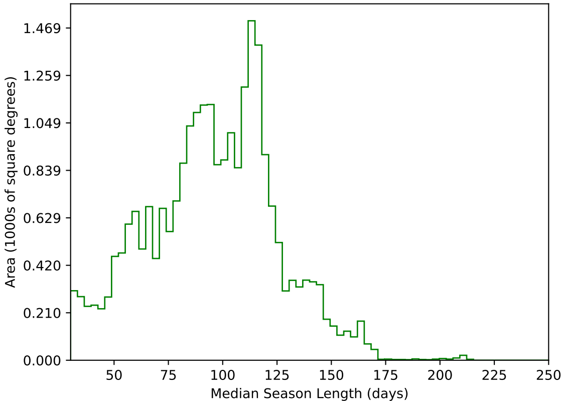
baseline_v3.3_10yrs All sky g band: Median Season Length
