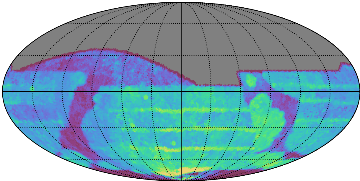
baseline_v3.3_10yrs All sky all bands: Median Season Length
