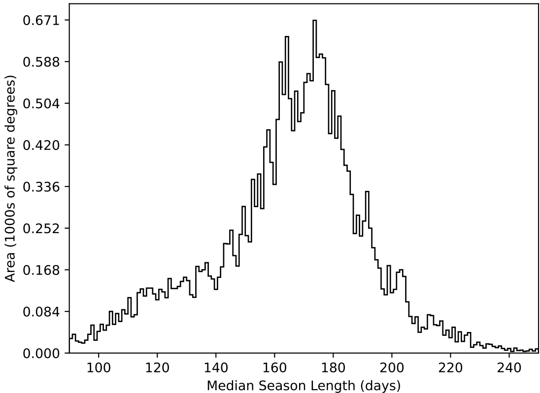
baseline_v3.3_10yrs All sky all bands: Median Season Length
