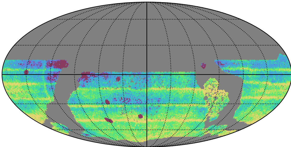
baseline_v3.3_10yrs WFD: Median Intra-Night Gap
