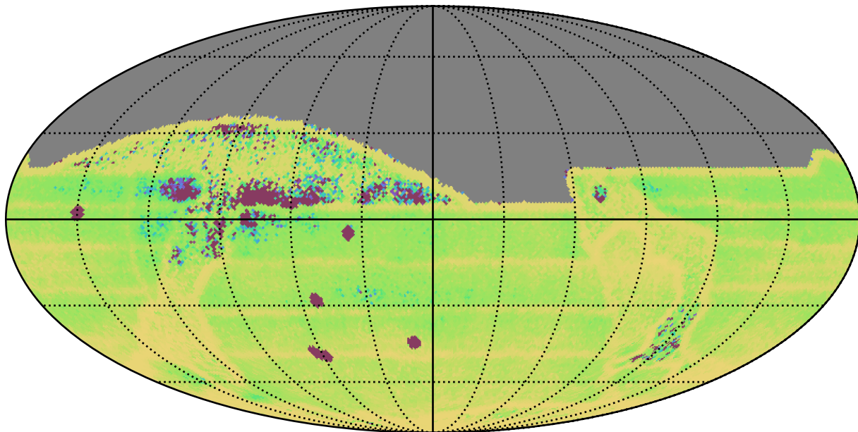
baseline_v3.3_10yrs All sky: Median Intra-Night Gap
