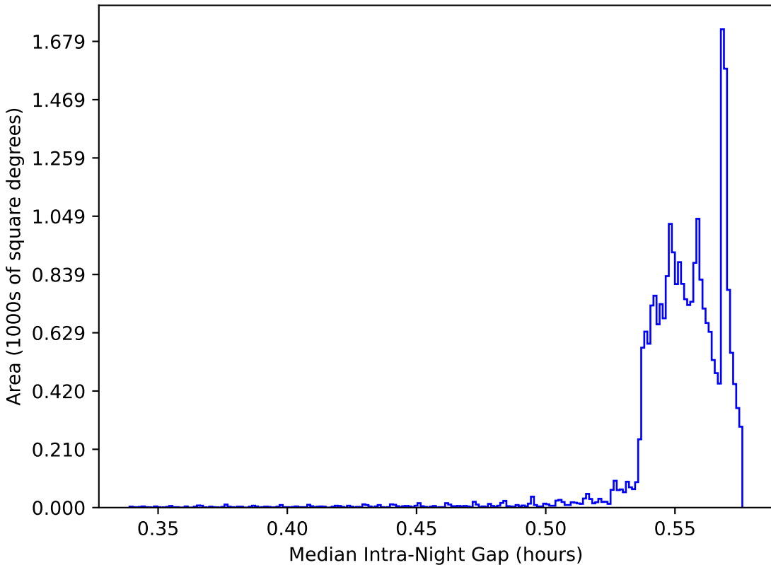
baseline_v3.3_10yrs All sky: Median Intra-Night Gap
