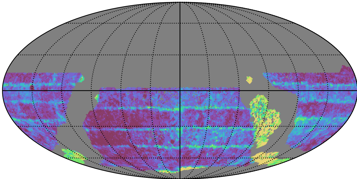
baseline_v3.3_10yrs WFD z band: Median Inter-Night Gap
